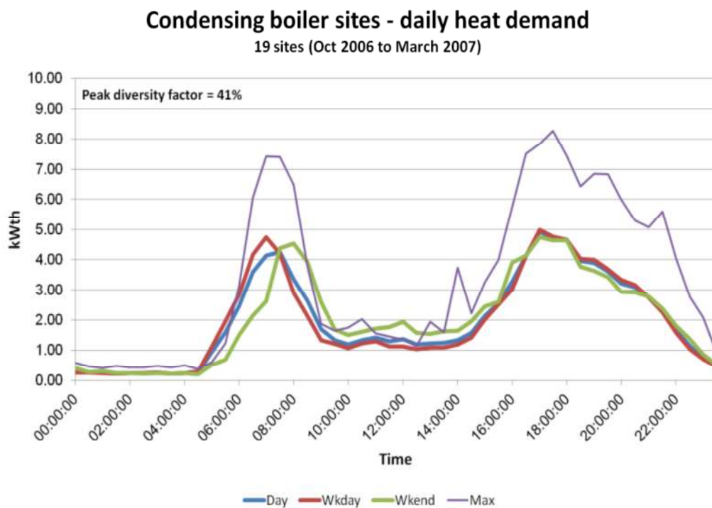
Figure 4a: Daily variation in space heating demand (from Sansom, 2015)
