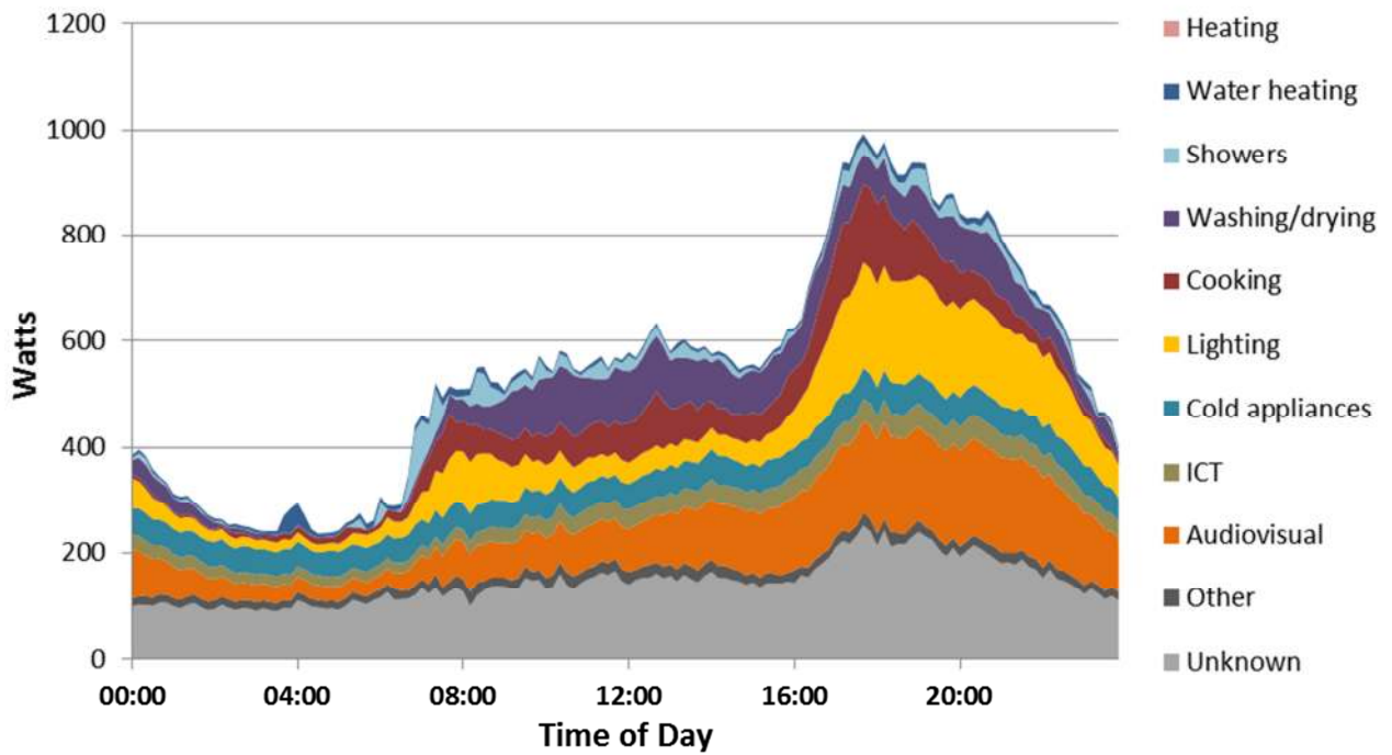
Figure 8a: Average winter (January) electrical demand for households without electric space heating (DECC, 2012a).
