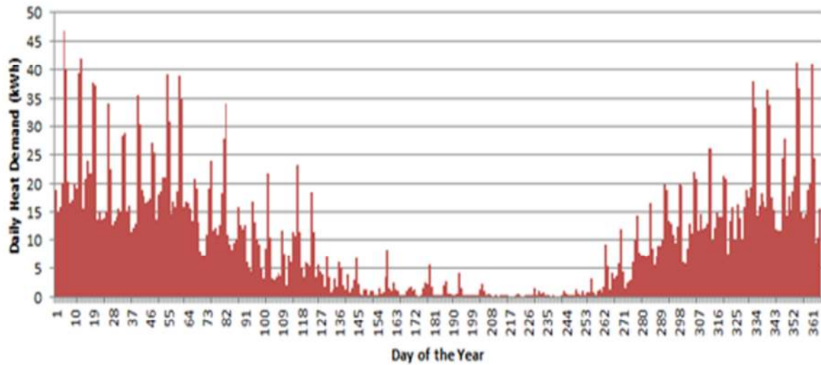
Figure 4b: Typical seasonal variation in space heating demand.
