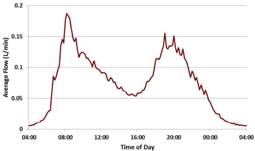
Figure 5: Average variation in hot water demand (based on EST (2008) data)
