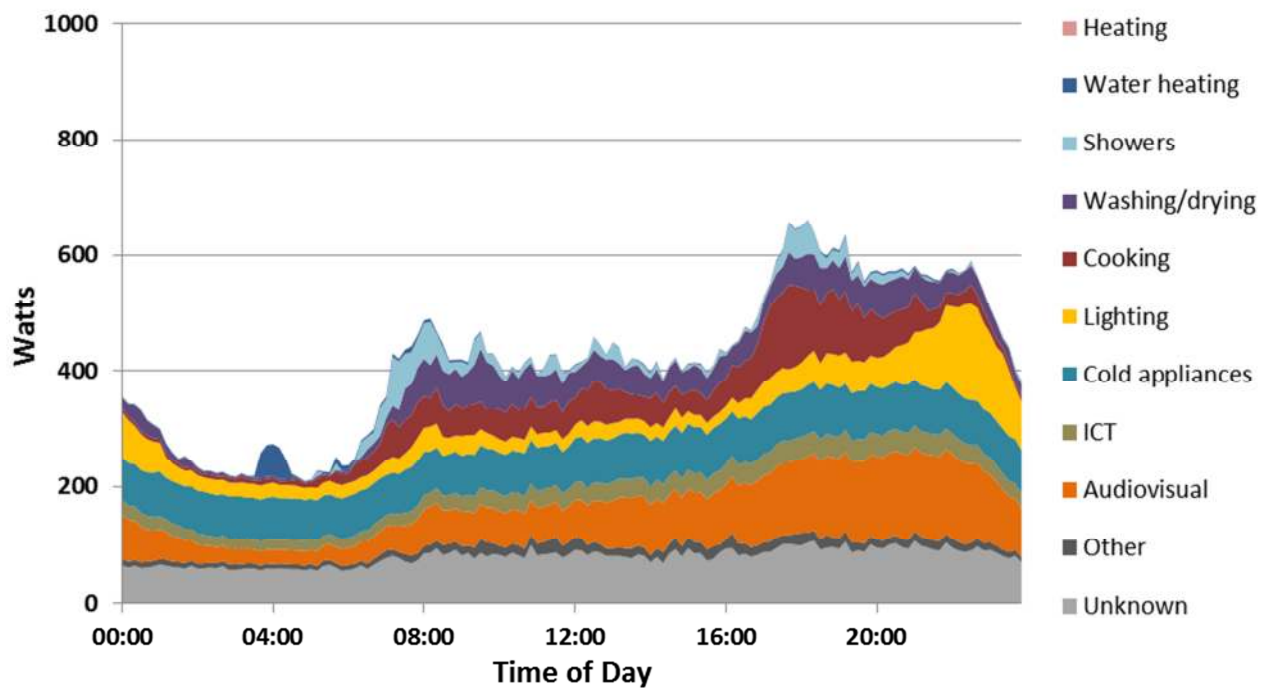
Figure 8b: Average winter (July) electrical demand for households without electric space heating (DECC, 2012a).
