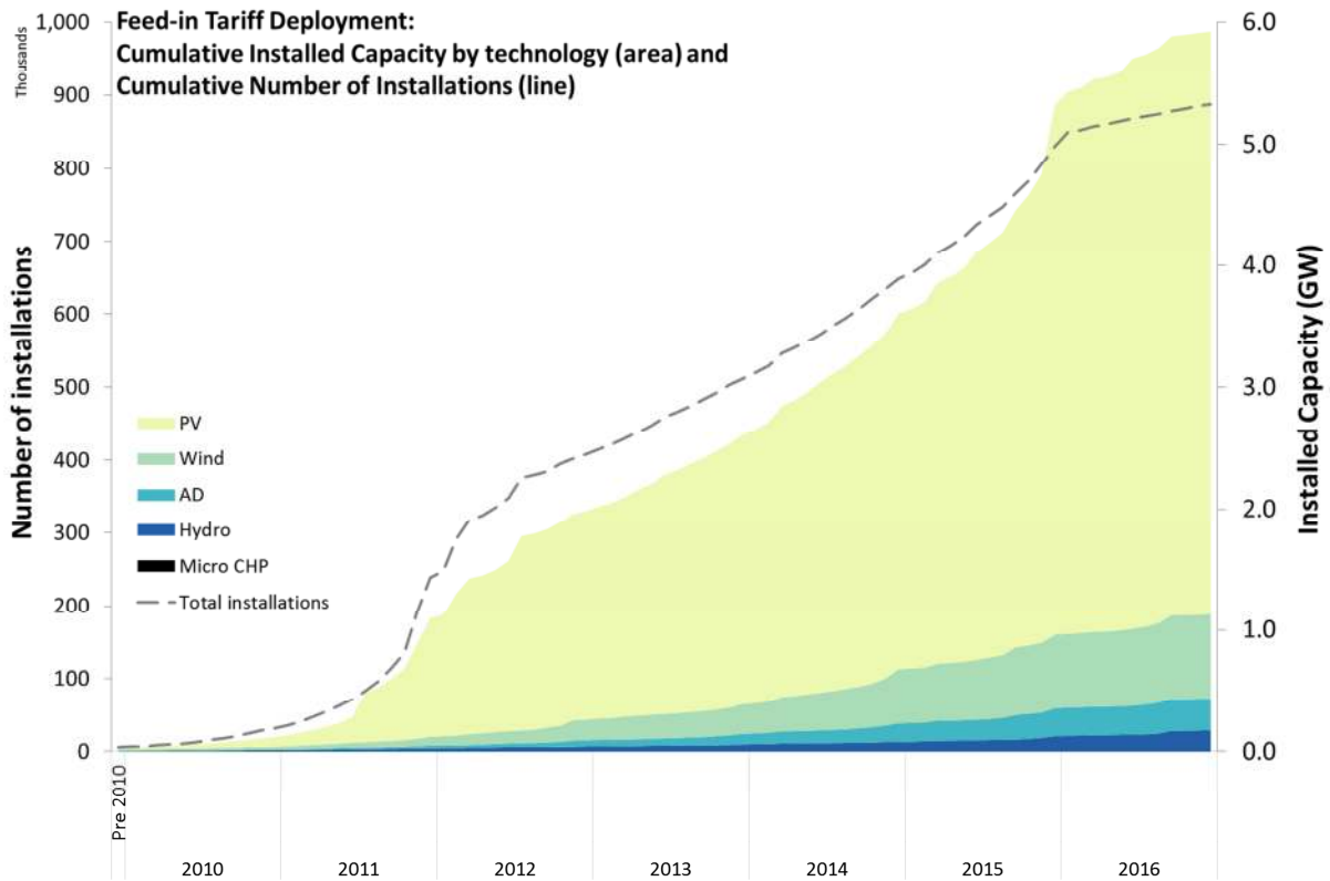
Figure 9: Cumulative feed-in tariff (FIT) installations since the launch of the FIT scheme (DBEIS, 2017b).
