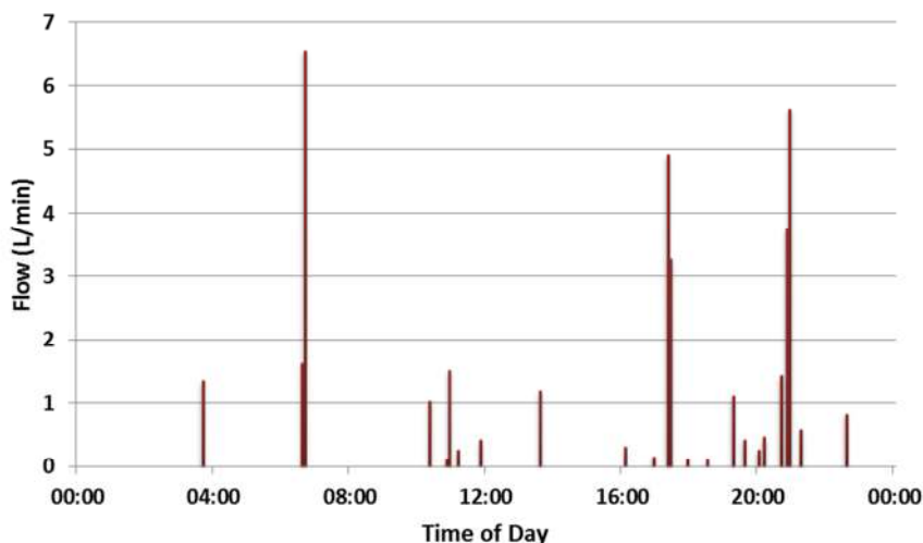
Figure 6: 'Typical' European daily hot water draw profile for 2-3 Person household (Knight and Ribberink, 2007).
